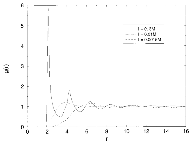
FIGURE 9 Radial distribution function as a function of particle separation, r , for three different ionic strengths and n_{\text{ins}} = 1000 .
