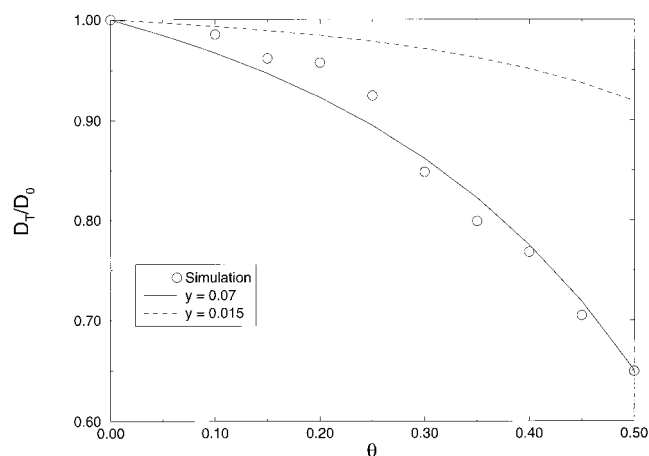
FIGURE 14 Relative diffusion coefficient, D_T/D_0 , where D_0 is the zero-coverage surface diffusion coefficient, against surface coverage for I = 0.3 \text{ M} . The solid and dashed lines show Minton's model (Eq. 9).
